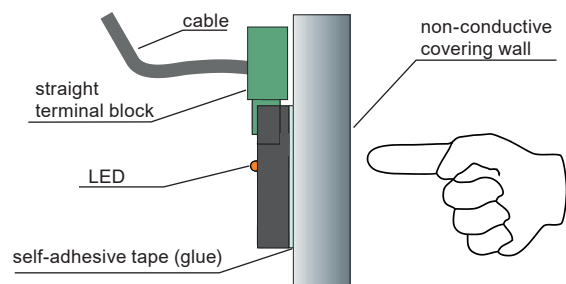
Fig. 2: CTS-41_-1 sensor installation
